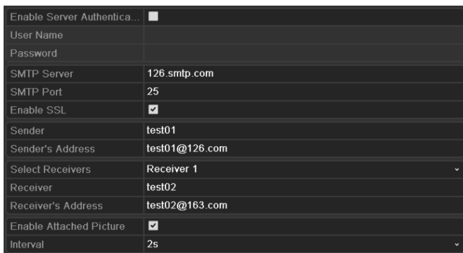
Figure 9. 24 Email Settings Interface
