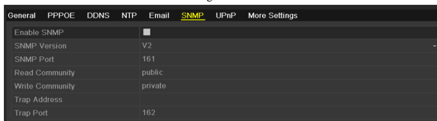
Figure 9.13 SNMP Settings Interface
