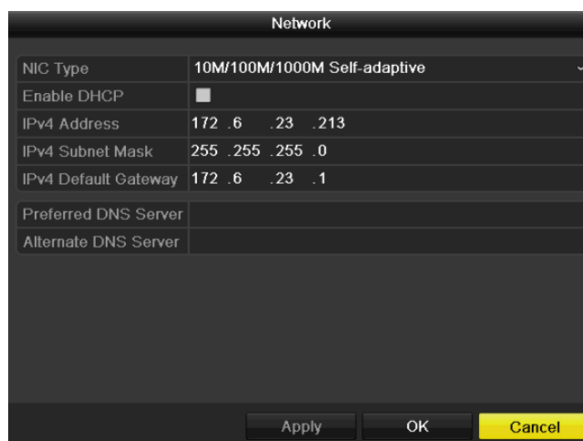
Figure 9. 33 Network Parameters Configuration
