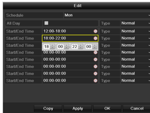
Figure 5. 8 Edit Schedule- Set Time Period
