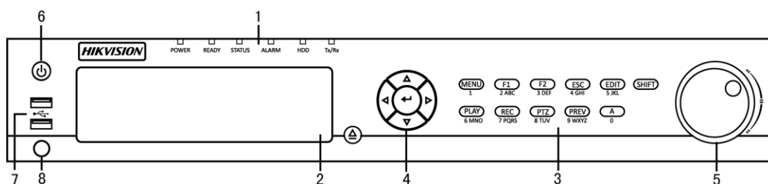
Figure 1. 4 Front Panel of DS-7300HFHI-ST
