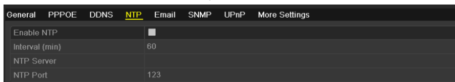
Figure 9.12 NTP Settings Interface
