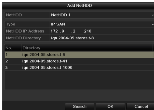
Figure 10. 8 Add IP SAN Disk
