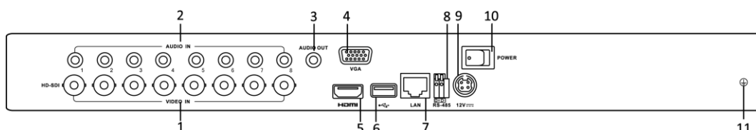
Figure 1. 10 DS-7208HFHI-SE and DS-7208HFHI-ST
