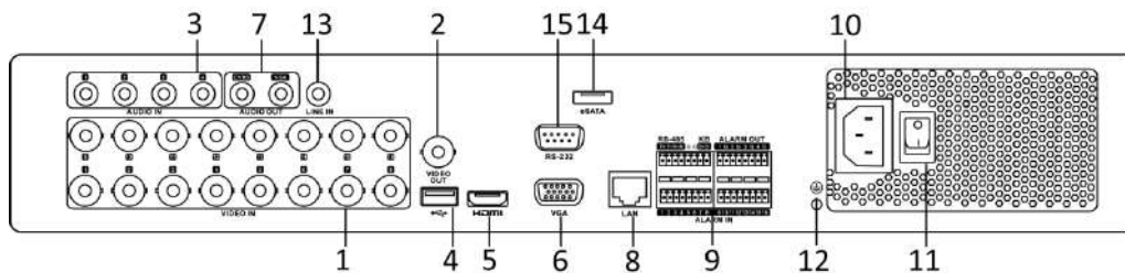
Figure 1-21 Rear Panel of DS-7300HQHI-K (with 16 Video Inputs)
