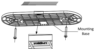
Figure 2-3 Fix the Mounting Base
